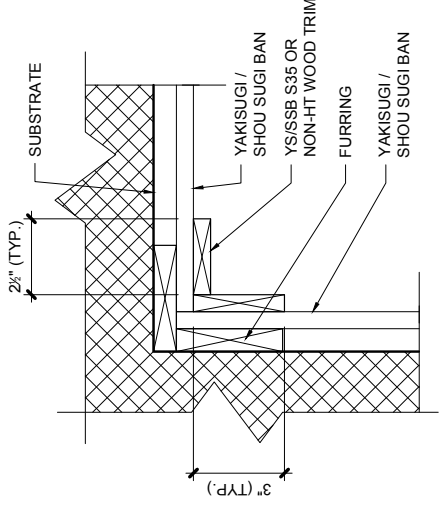
A PLAN VIEW INSIDE CORNER WOOD OPTIONS
