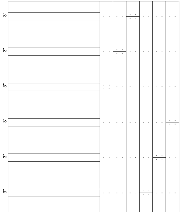
VERTICAL FURRING 3" MINIMUM FURRING WITH STAGGERED BUTTS
