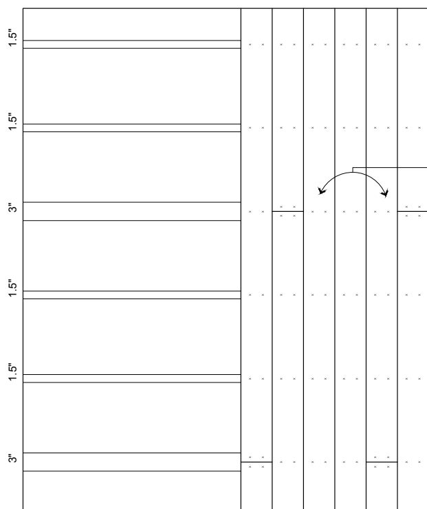
VERTICAL FURRING 3" MINIMUM FURRING WIDTH FOR BUTTS 1.5" MINIMUM FURRING WIDTH FOR INTERMEDIATE STRIPPING MINIMUM 2 UNBROKEN ROWS BETWEEN BUTTS FOR BEST APPEARANCE
