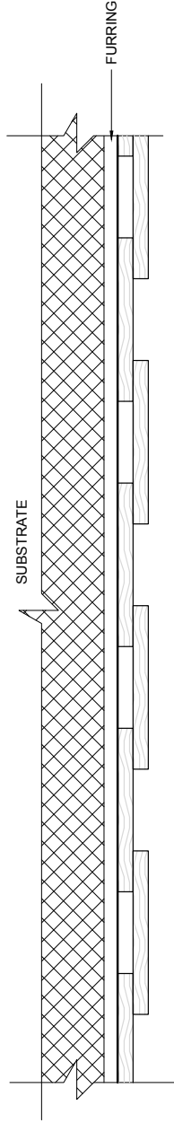
(A) VERTICAL BOARD & BATTEN
