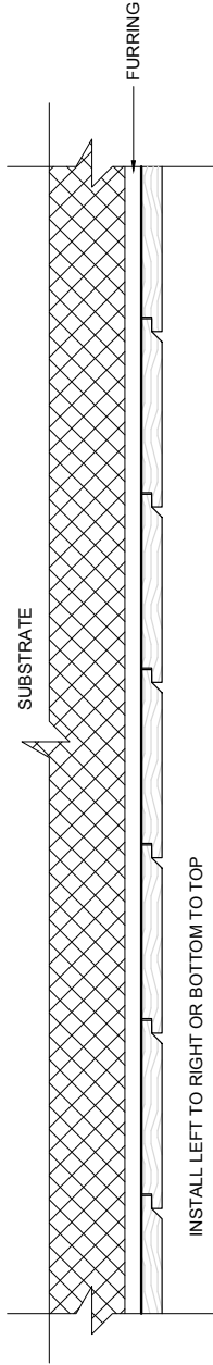
A SHIPLAP (VERTICAL OR HORIZONTAL)
