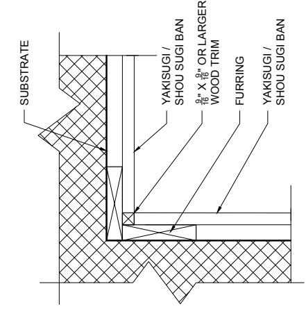
B PLAN VIEW INSIDE CORNER WOOD OPTIONS
