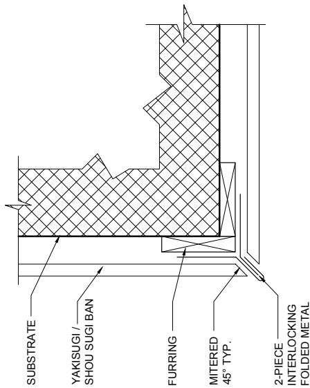
D PLAN VIEW - OUTSIDE CORNER - METAL
