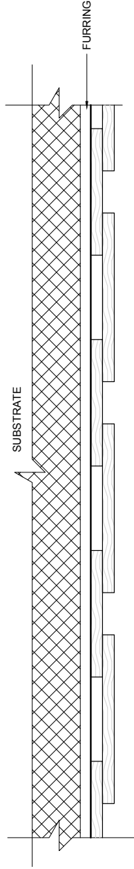
(B) VERTICAL BOARD & BATTEN
