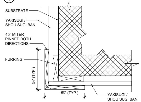
(C) PLAN VIEW - OUTSIDE CORNER - WOOD
