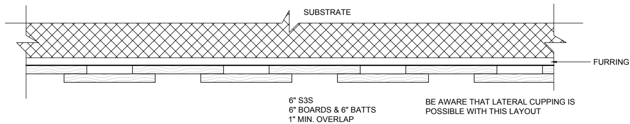
(B) VERTICAL BOARD & BATTEN
