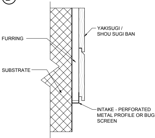
(E) HORIZONTAL INSTALL DRIP INTAKE
