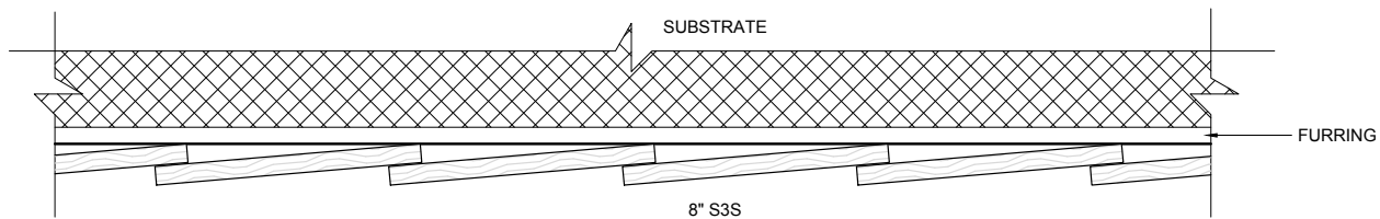
B 6" VERTICAL OR HORIZONTAL CLAPBOARD
