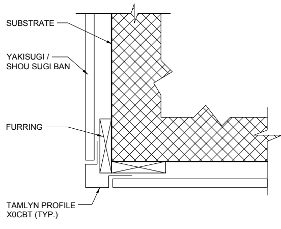
E PLAN VIEW - OUTSIDE CORNER - METAL
