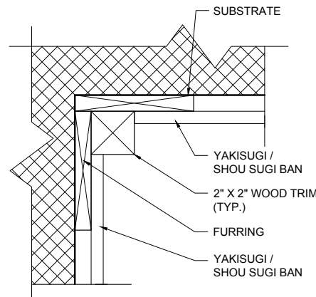
E PLAN VIEW INSIDE CORNER WOOD OPTIONS
