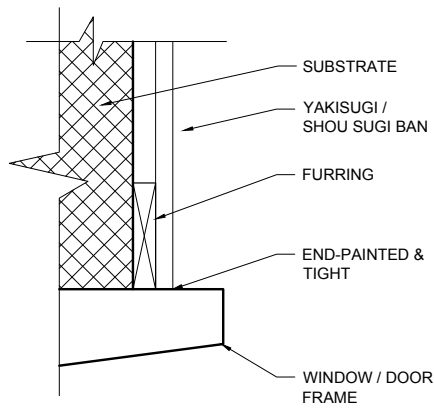
A PLAN VIEW - DOOR & WINDOW PENETRATION
