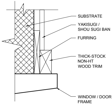
A PLAN VIEW - DOOR & WINDOW PENETRATION
