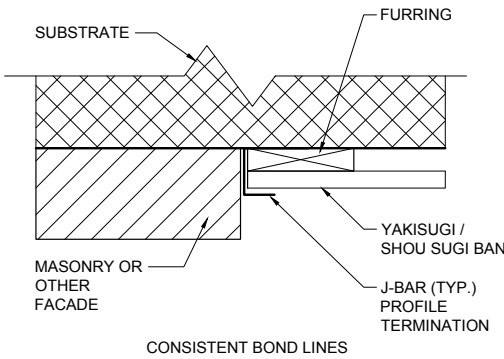
E PLAN VIEW - HORIZONTAL LAYOUT
