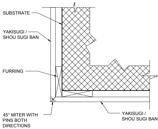
(A) PLAN VIEW - OUTSIDE CORNER - WOOD
