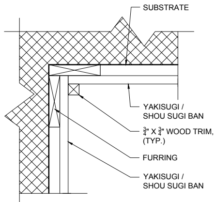
D PLAN VIEW INSIDE CORNER WOOD OPTIONS
