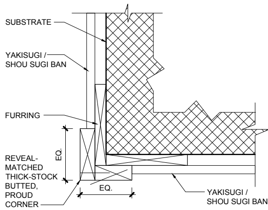
A PLAN VIEW - OUTSIDE CORNER - WOOD
