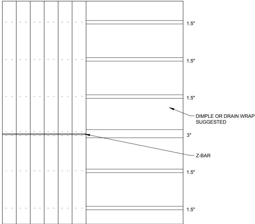
VERTICAL FURRING 3" MINIMUM FURRING WIDTH FOR BUTTS 1.5" MINIMUM FURRING WIDTH FOR INTERMEDIATE STRIPPING VENTED OUT CORNERS AND PENETRATIONS PLEASE USE Z-BAR AT BOND LINES
