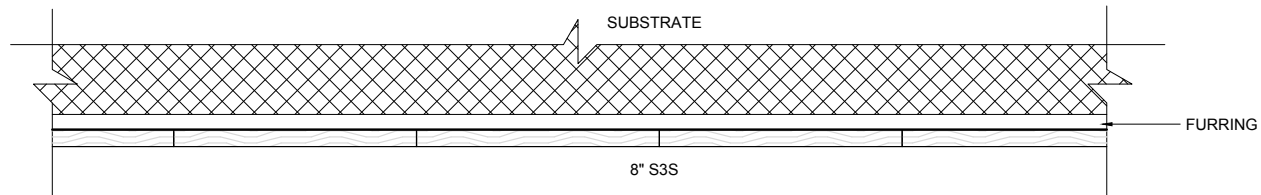
(C) 8" CLOSED SCREEN, 8" S3S
