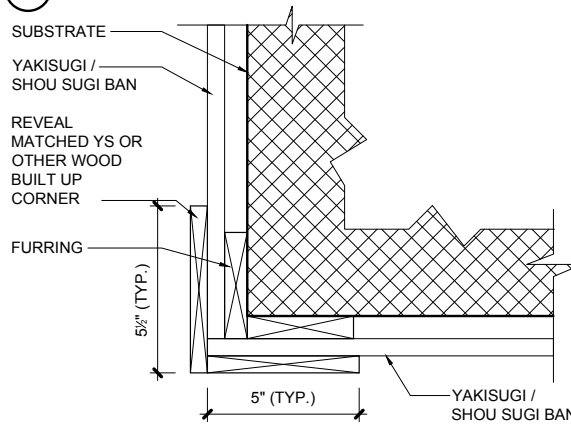
(B) PLAN VIEW - OUTSIDE CORNER - WOOD
