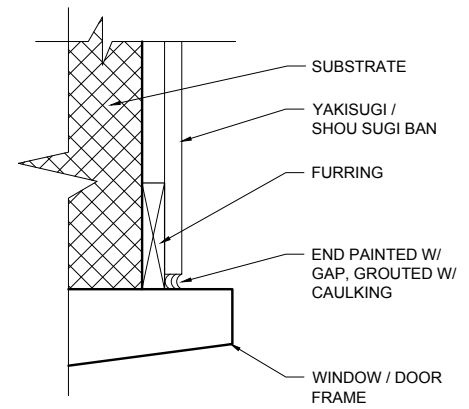
C PLAN VIEW - DOOR & WINDOW PENETRATION
