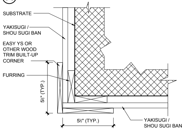
(A) PLAN VIEW - OUTSIDE CORNER - WOOD
