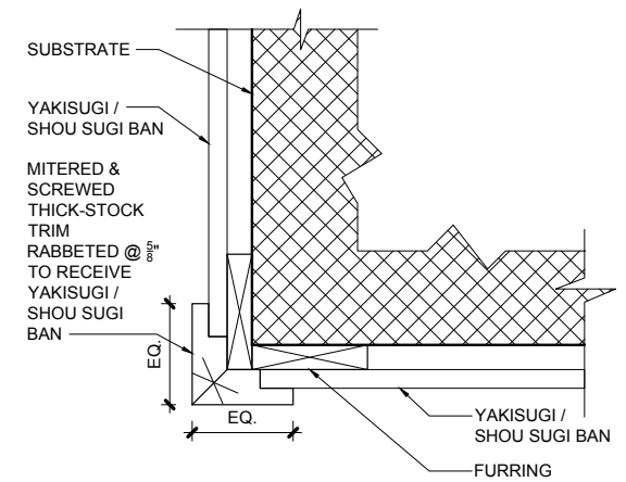
C PLAN VIEW - OUTSIDE CORNER - WOOD
