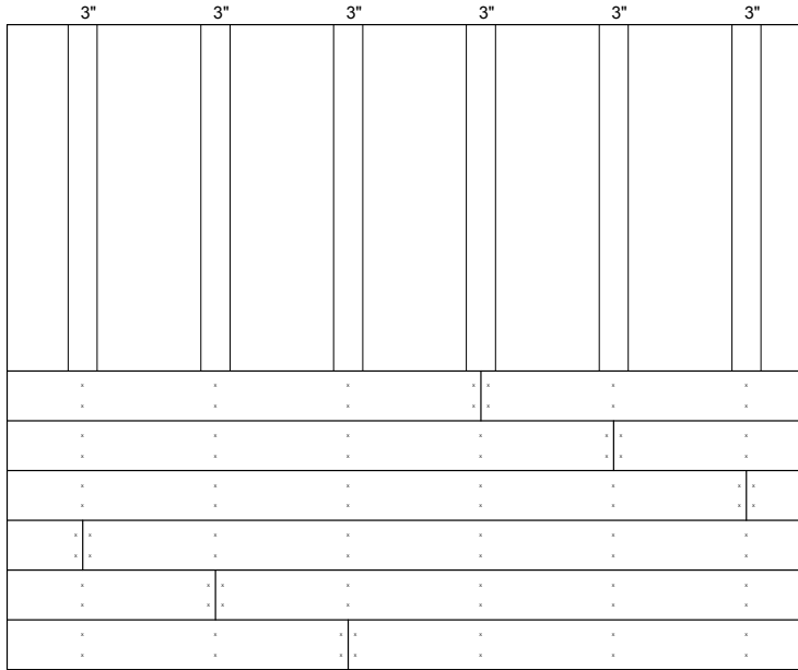
VERTICAL FURRING 3" MINIMUM FURRING WITH STAGGERED BUTTS
