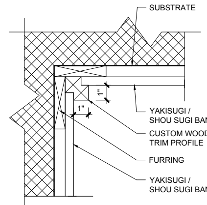
F PLAN VIEW INSIDE CORNER WOOD OPTIONS
