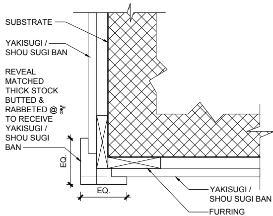
D PLAN VIEW - OUTSIDE CORNER - WOOD
