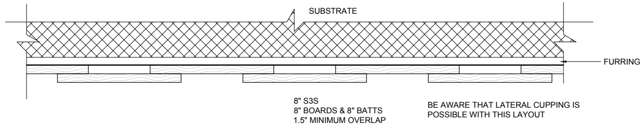
(A) VERTICAL BOARD & BATTEN
