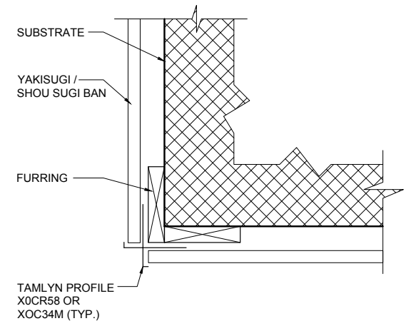
F PLAN VIEW - OUTSIDE CORNER - METAL
