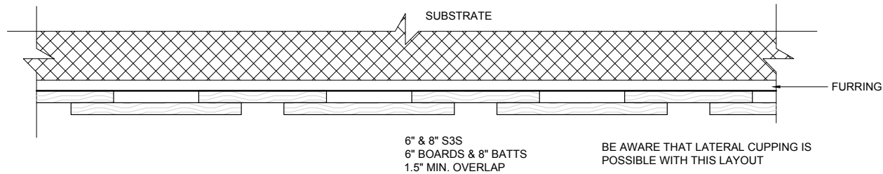
(C) VERTICAL REVERSE BOARD & BATTEN
