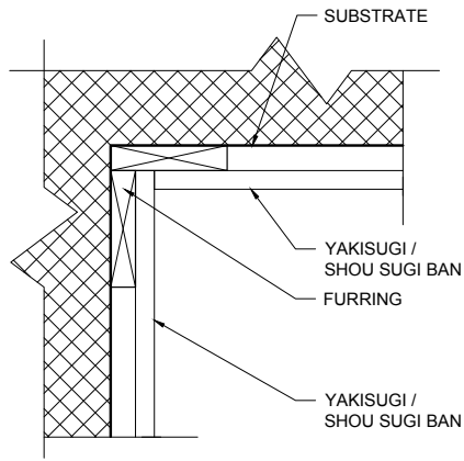
A PLAN VIEW INSIDE CORNER WOOD OPTIONS
