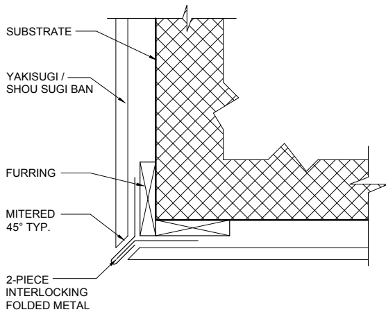
D PLAN VIEW - OUTSIDE CORNER - METAL
