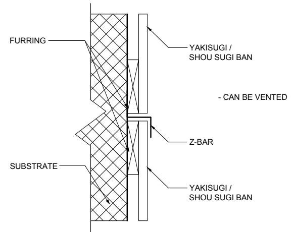
(C) VERTICAL LAYOUT BUTT JOINT
