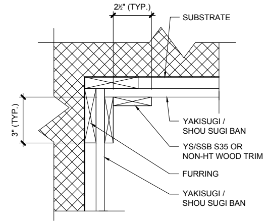
C PLAN VIEW INSIDE CORNER WOOD OPTIONS
