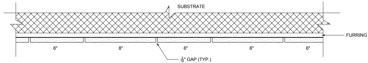
(C) 6" & 8" OPEN SCREEN, 6" & 8" S3S
