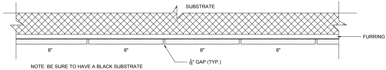
(A) 8" OPEN SCREEN, 8" S3S
