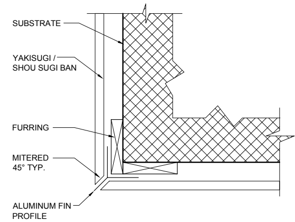
C PLAN VIEW - OUTSIDE CORNER - METAL
