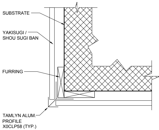
A PLAN VIEW - OUTSIDE CORNER - METAL
