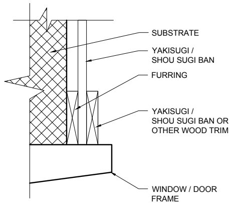
D PLAN VIEW - DOOR & WINDOW PENETRATION
