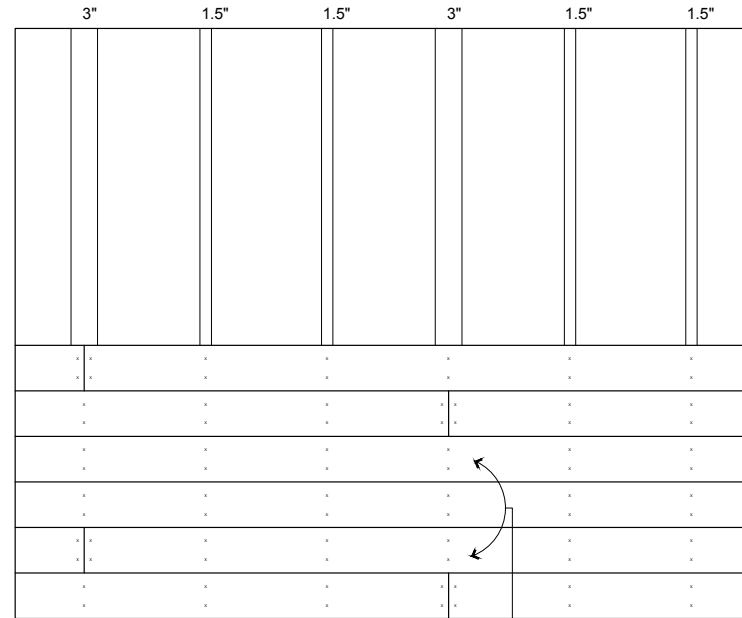
VERTICAL FURRING 3" MINIMUM FURRING WIDTH FOR BUTTS 1.5" MINIMUM FURRING WIDTH FOR INTERMEDIATE STRIPPING
