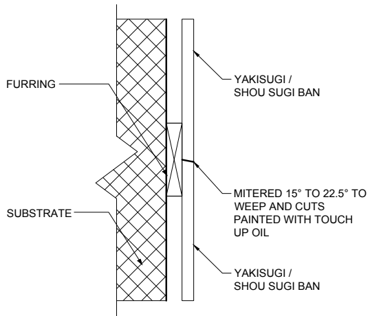
(A) VERTICAL LAYOUT SCARF JOINT
