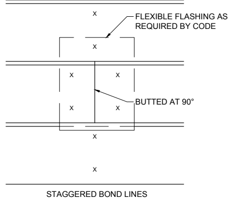
B HORIZONTAL LAYOUT BUTT JOINT
