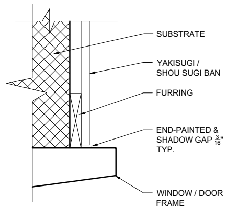
B PLAN VIEW - DOOR & WINDOW PENETRATION
