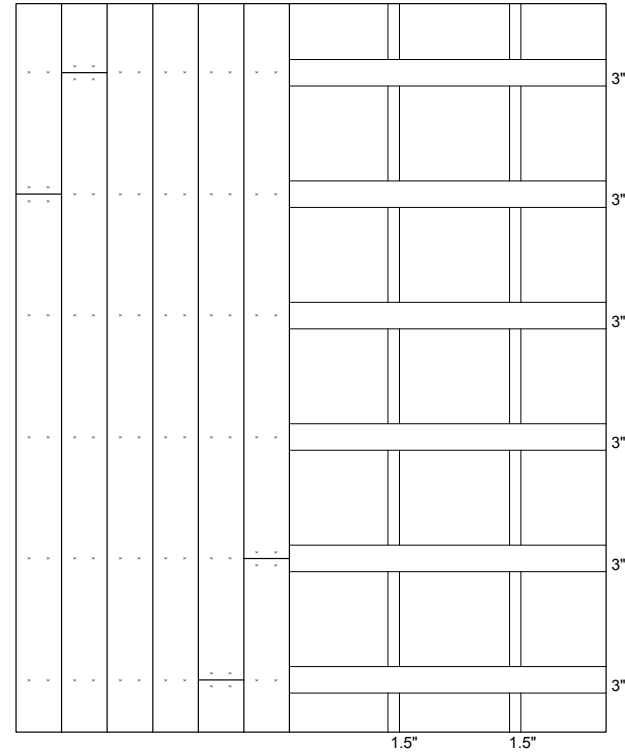
GRID FURRING (REQUIRED BY SOME MUNICIPALITIES)
