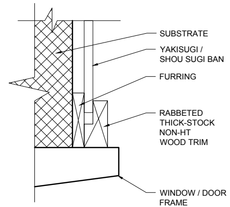
F PLAN VIEW - DOOR & WINDOW PENETRATION
