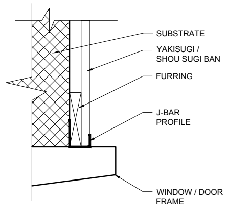
E PLAN VIEW - DOOR & WINDOW PENETRATION
