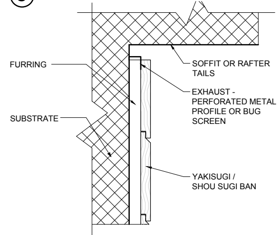
(F) VENTING AT SOFFIT OR RAFTER
