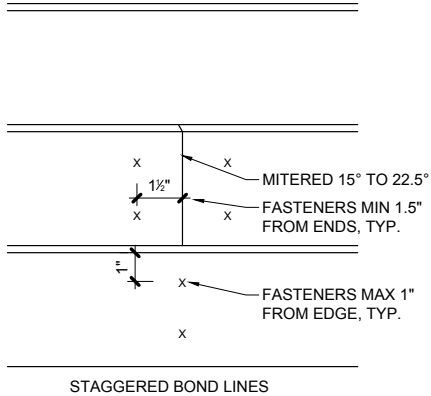
A HORIZONTAL LAYOUT SCARF JOINT
