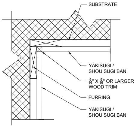
B PLAN VIEW INSIDE CORNER WOOD OPTIONS
