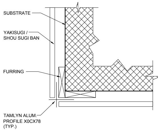
B PLAN VIEW - OUTSIDE CORNER - METAL
