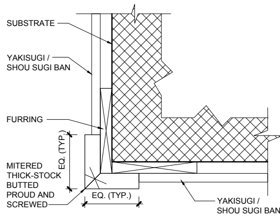
B PLAN VIEW - OUTSIDE CORNER - WOOD
