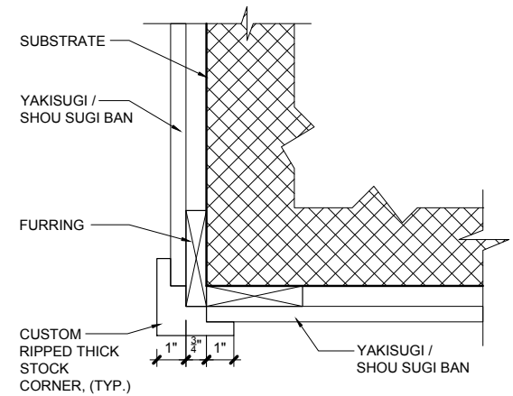
(C) PLAN VIEW - OUTSIDE CORNER - WOOD
